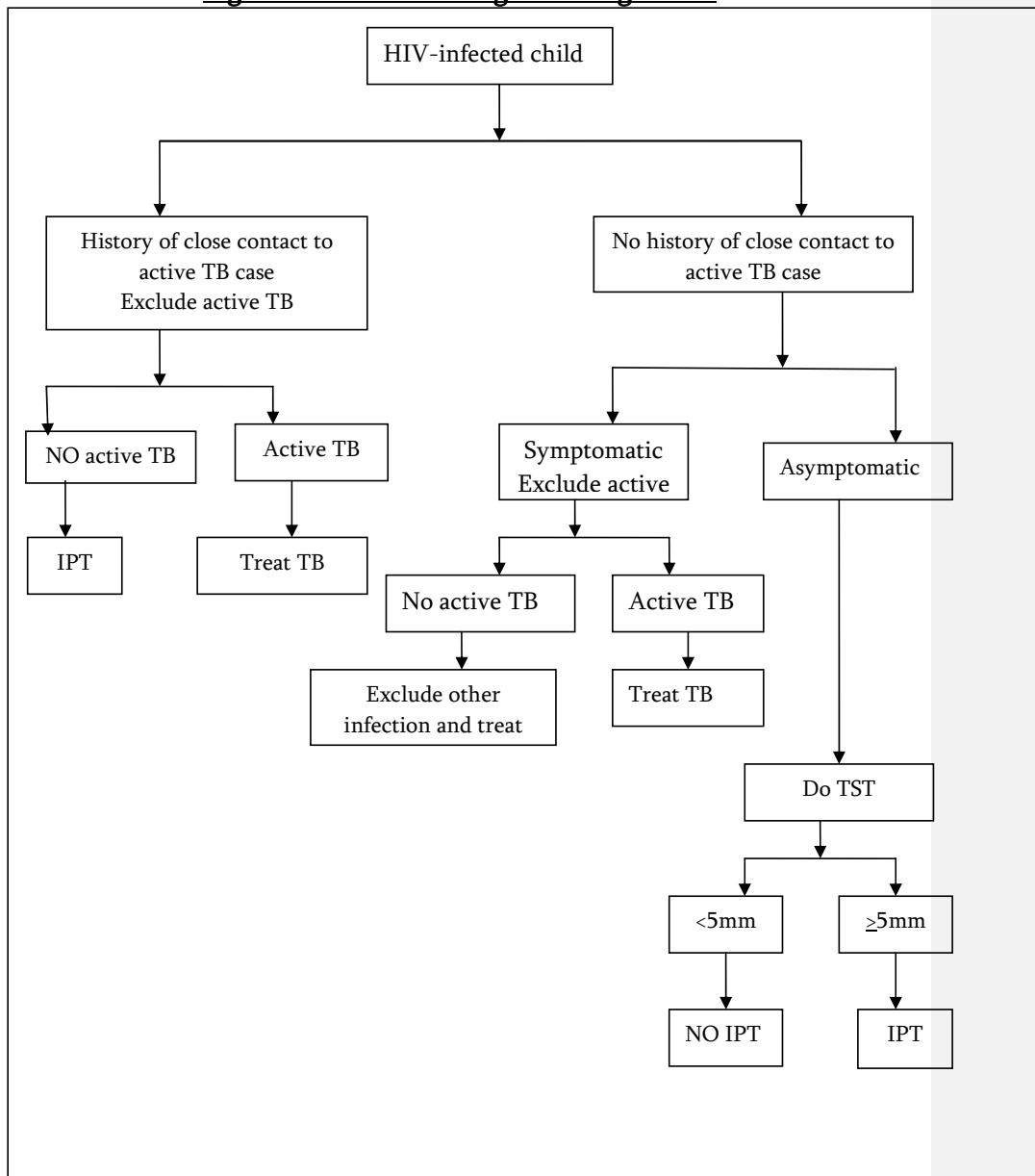
Figure 5.1Draft IPT Diagnostic Algorithm
