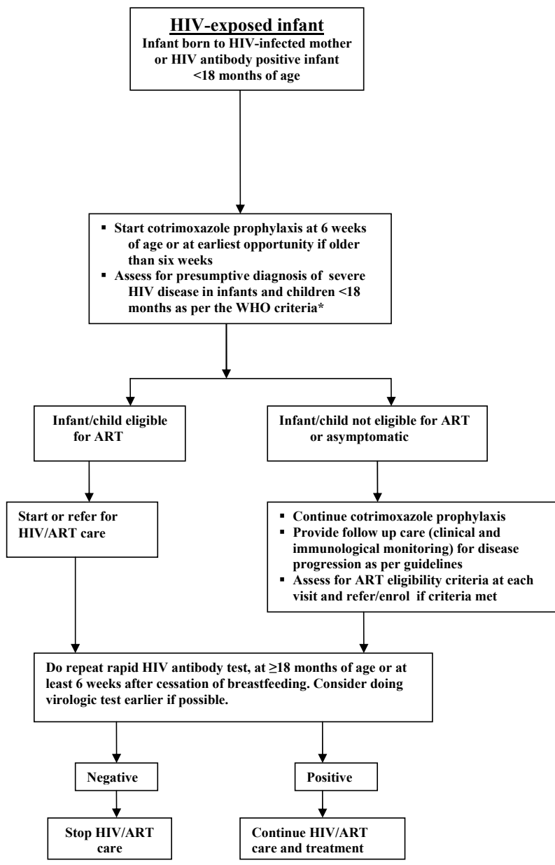
Figure 2.2 Diagnostic Algorithm for Infants <18 Months of Age Where Virological Tests are Unavailable
